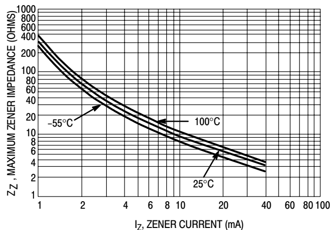
Figure 7. Variation of Zener Impedance With Current and Temperature (1N821 Series)
