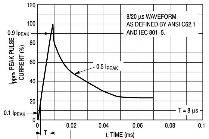
Figure 12. Pulse Waveform
