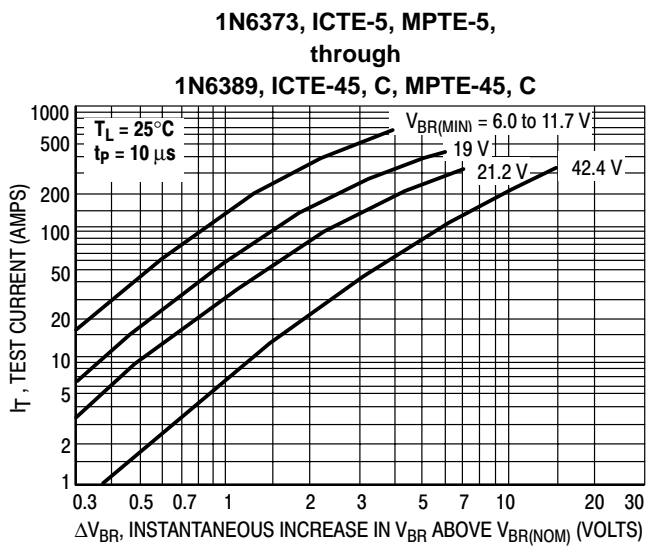
Figure 6. Dynamic Impedance
