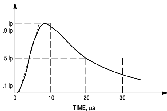
Figure 6. Pulse Waveform ( 8/20 \mu\text{s} )
