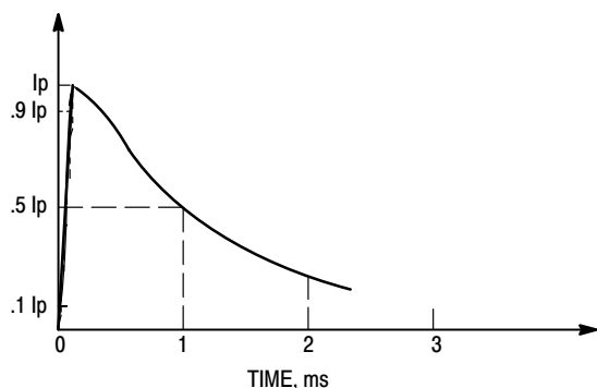
Figure 5. Pulse Waveform ( 10/1000 \mu\text{s} )
